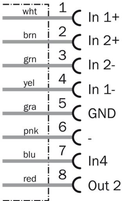
Connection diagram, Encoder connection
